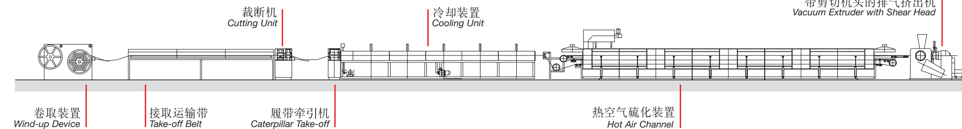
GS Vak型排气挤出机 Vacuum extruder type GS Vak
