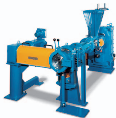
挤出机-齿轮泵机组 Extruder-Gear pump combination
